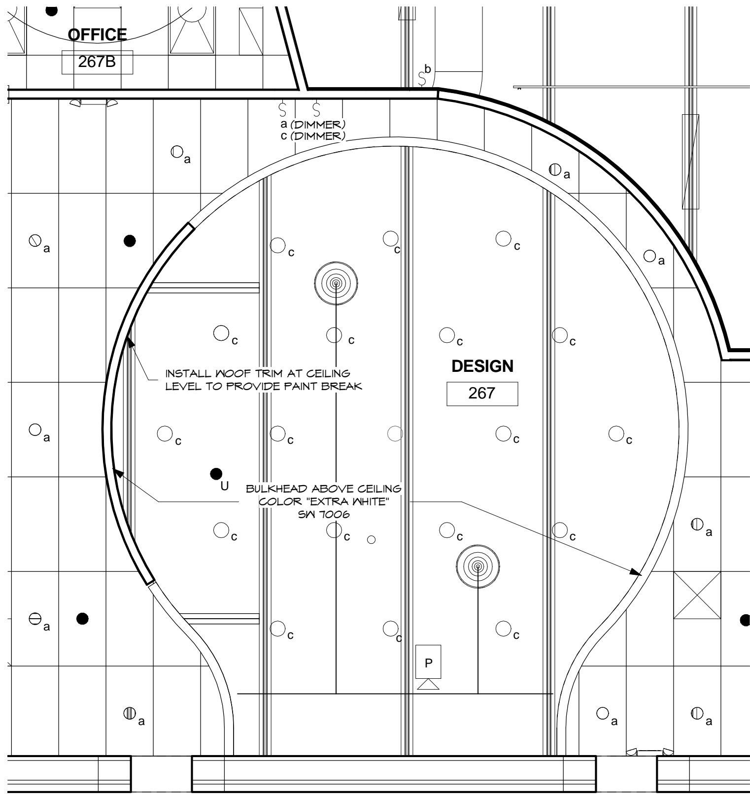
2 REFLECTED CEILING PLAN 1/4" = 1'-0"
